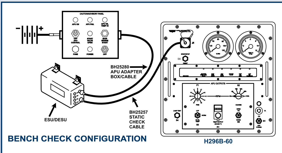
Simulates APU signals and sequences in back shop environment to verify proper ESU/DESU operation.
