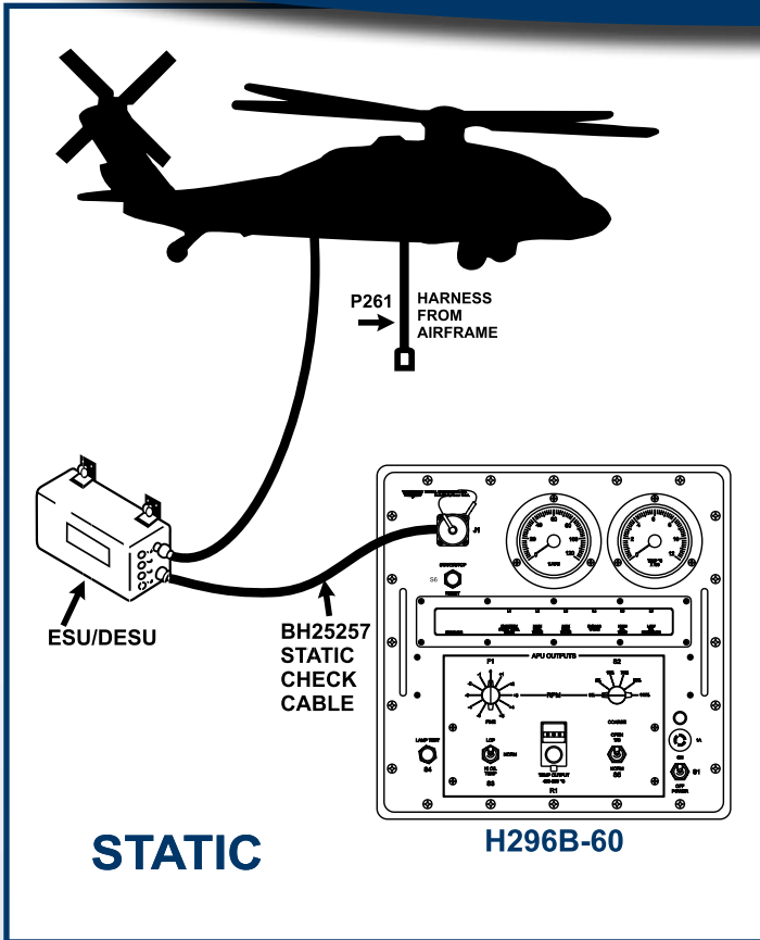
Simulates APU signals and sequences to verify proper ESU/DESU operation.
