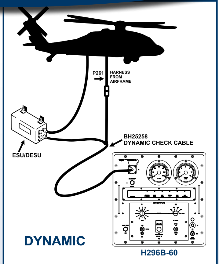
Monitors the signals between the APU, ESU/DESU and Cockpit Advisory Panel to verify operational signals and sequences.
